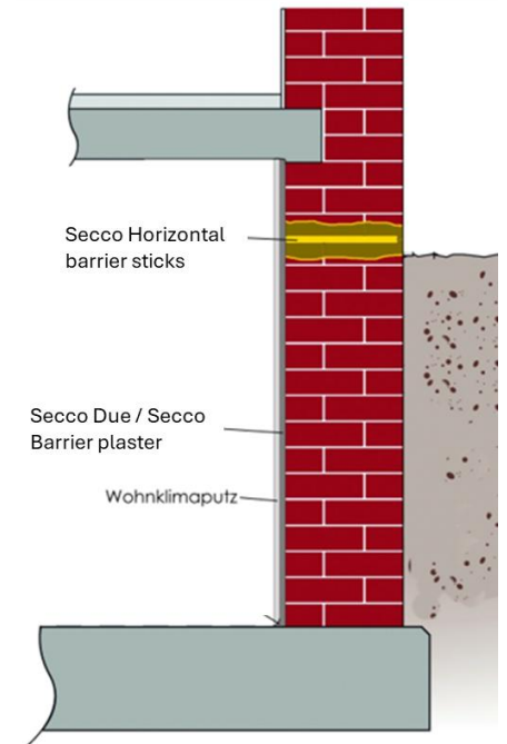
System overview of internal waterproofing
